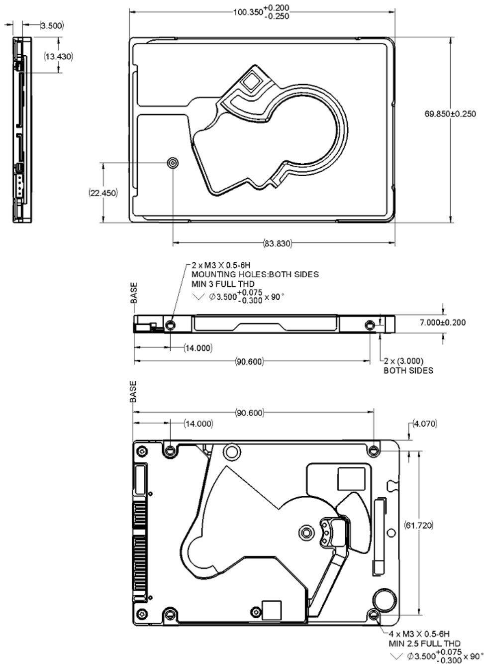
Figure 4 Mounting Dimensions
